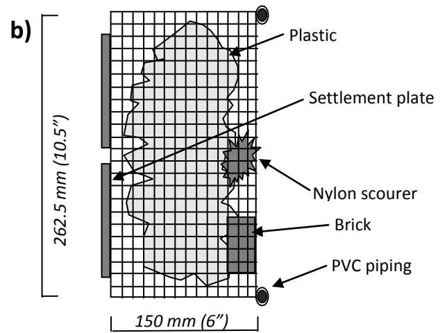
Figure 2: Design of sampling devices to capture invertebrates using engineered shorelines as habitat. a) Front view of the sampling device (facing away from the shoreline), where tiles (4, 1 each of timber, ceramic, stone and acrylic) will be attached to a cage to allow colonization of sessile invertebrates that occupy the water column as larvae. Each sampling device will be lowered below the water line at low tide and attached to a stable anchorage point on the shoreline using rope, with PVC piping attached to the cage for stability. b) Side view of the sample device showing cage mesh netting and scourers, which will allow colonization of mobile invertebrates and bivalve recruits, respectively. A brick is also included to both stabilize the device and to provide additional surfaces for settlement and colonization. Each sampling device will be submerged for 8 weeks to allow colonization of a well-developed assemblage.
