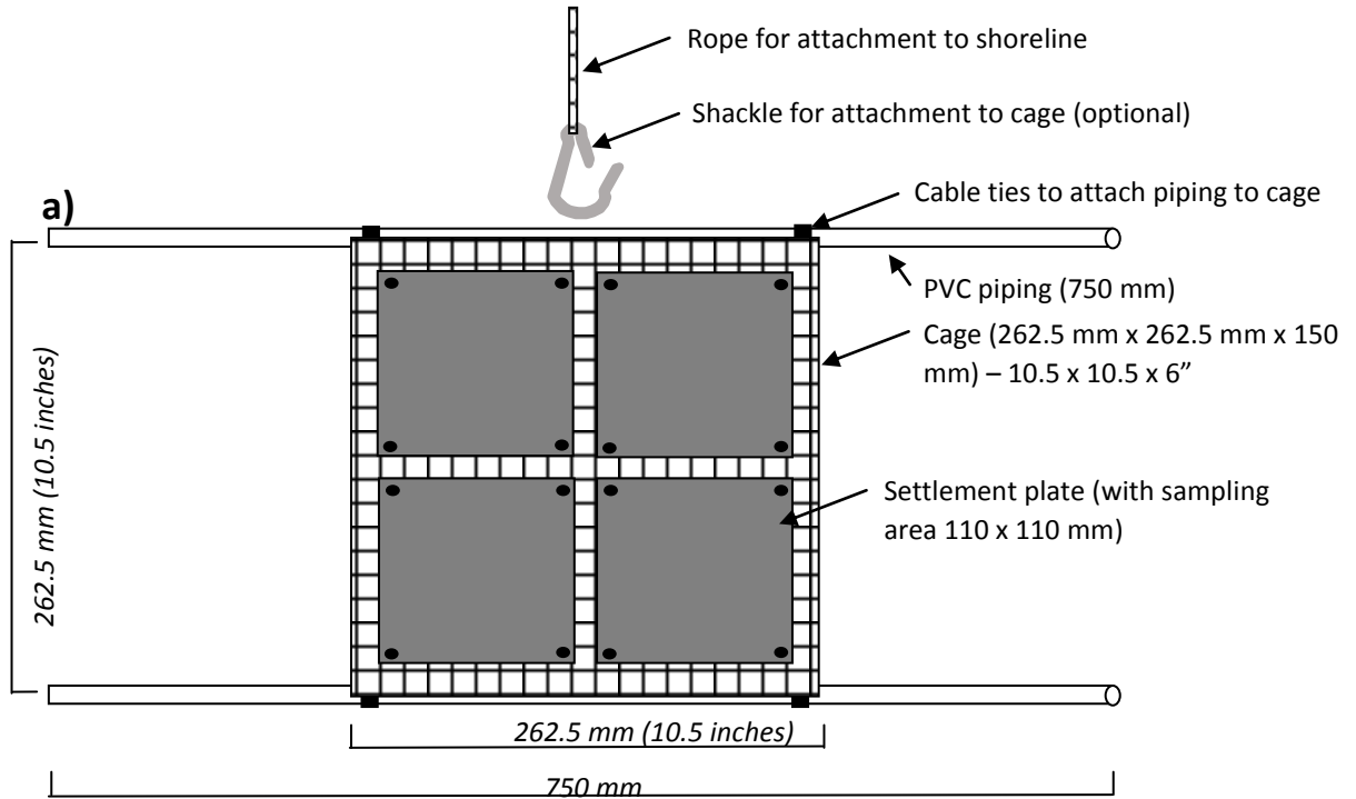
Figure 2: Design of sampling devices to capture invertebrates using engineered shorelines as habitat. a) Front view of the sampling device (facing away from the shoreline), where tiles (4, 1 each of timber, ceramic, stone and acrylic) will be attached to a cage to allow colonization of sessile invertebrates that occupy the water column as larvae. Each sampling device will be lowered below the water line at low tide and attached to a stable anchorage point on the shoreline using rope, with PVC piping attached to the cage for stability. b) Side view of the sample device showing cage mesh netting and scourers, which will allow colonization of mobile invertebrates and bivalve recruits, respectively. A brick is also included to both stabilize the device and to provide additional surfaces for settlement and colonization. Each sampling device will be submerged for 8 weeks to allow colonization of a well-developed assemblage.
